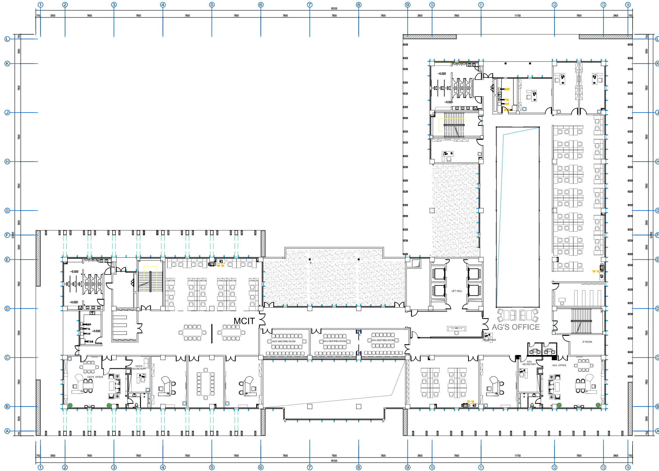
LEVEL 6 SCALE:1:350
